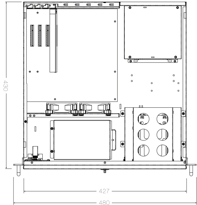
MECHANICAL DRAWING
