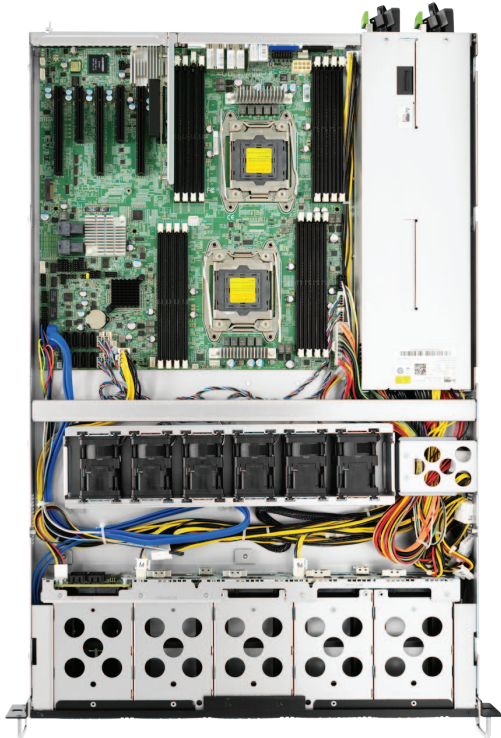
(Power supply is optional. Motherboard is not included.)
