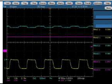
90Vac, 5kHz, 50% Duty, 12Vsb@2~3A;12V@0.5A, CH1:+12Vsb current, CH2:+12Vsb, CH3:PG
