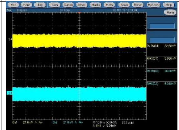
264Vac/63Hz Min Load CH1: +12V, CH2: +12Vsb
