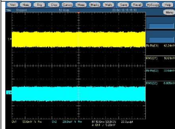
264Vac/63Hz Cross Load 1 CH1: +12V, CH2: +12Vsb
