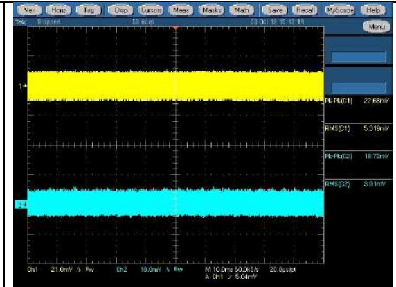
90Vac/47Hz Cross Load 2 CH1: +12V, CH2: +12Vsb
