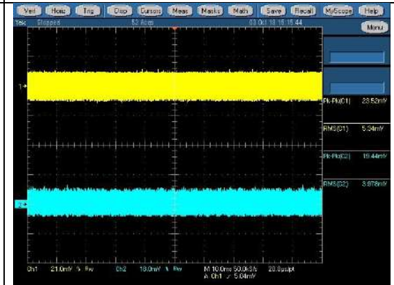
264Vac/63Hz Cross Load 2 CH1: +12V, CH2: +12Vsb
