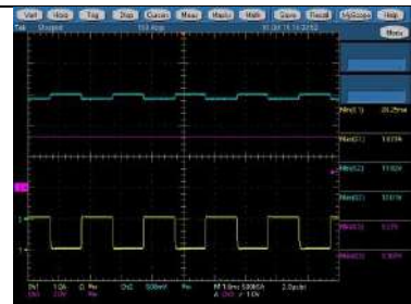
264Vac, 500Hz, 50% Duty, 12Vsb@0.1~1.1A;12V@44.73A, CH1:+12Vsb current, CH2:+12Vsb, CH3:PG
