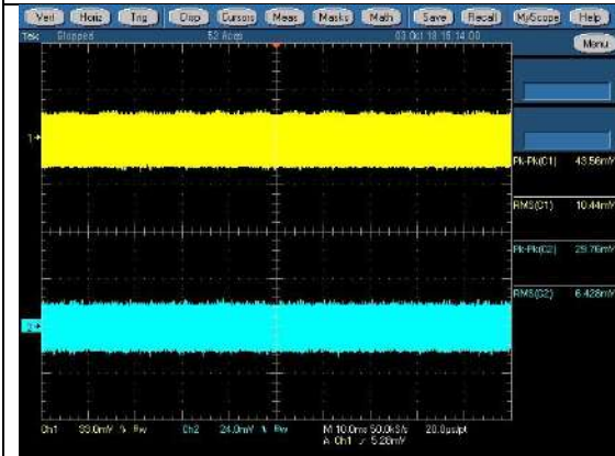
264Vac/63Hz Max Load CH1: +12V, CH2: +12Vsb
