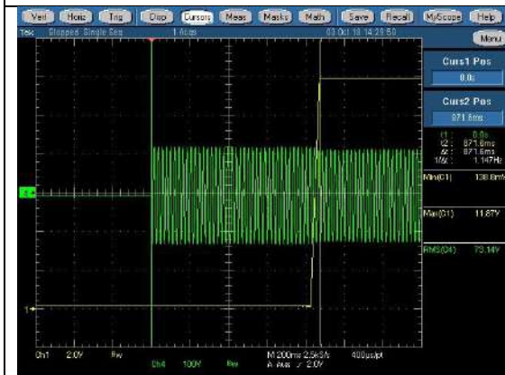
90V +12V max CH1:+12V, CH4:Vin
