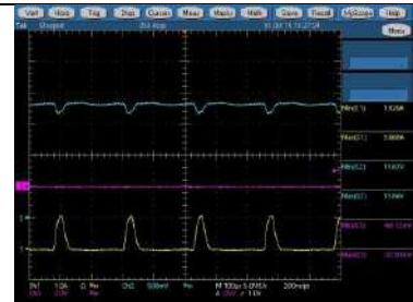
264Vac, 5kHz, 10% Duty, 12Vsb@2~ 3A;12V@OFF, CH1:+12Vsb current, CH2:+12Vsb, CH3:PG
