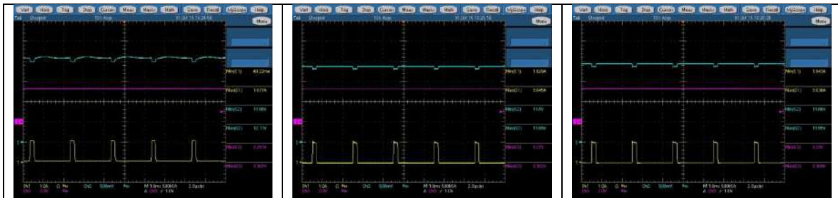
264Vac, 500Hz, 10% Duty, 12Vsb@0.1~ 1.1A;12V@0.5A, CH1:+12Vsb current, CH2:+12Vsb, CH3:PG
