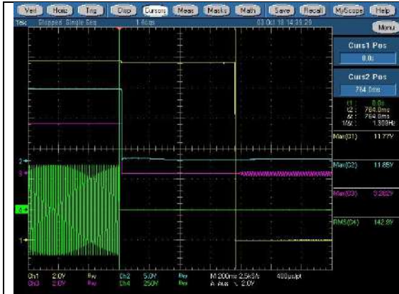
264V +12Vsb max CH1:+12Vsb, CH2:+12V, CH3:PG, CH4:Vin
