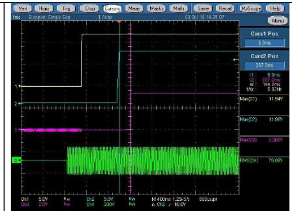
AC ON_90V +12V min CH1:+12Vsb, CH2:+12V, CH3:PG, CH4:Vin
