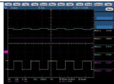
264Vac, 50Hz, 50% Duty, 12Vsb@2~3A;12V@42.83A, CH1:+12Vsb current, CH2:+12Vsb, CH3:PG
