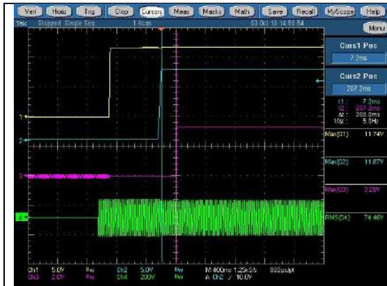
AC ON_90V +12V max CH1:+12Vsb, CH2:+12V, CH3:PG, CH4:Vin
