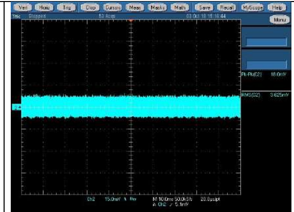
264Vac/63Hz Standby Mode CH2: +12Vsb
