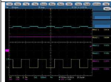
264Vac, 50Hz, 50% Duty, 12Vsb@2~3A;12V@0.5A, CH1:+12Vsb current, CH2:+12Vsb, CH3:PG
