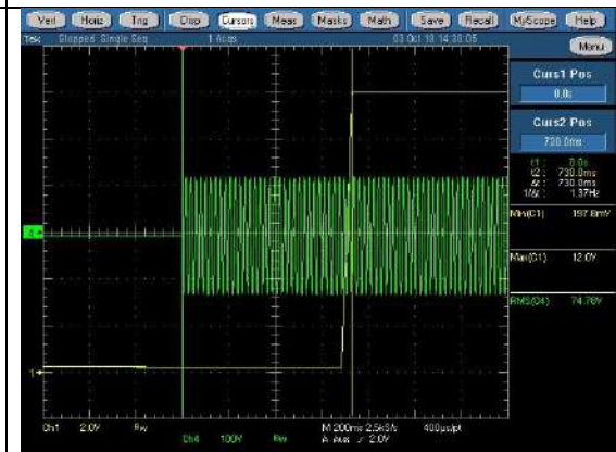
90V +12V min CH1:+12V, CH4:Vin
