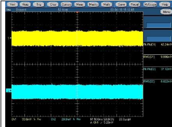
90Vac/47Hz Cross Load 1 CH1: +12V, CH2: +12Vsb
