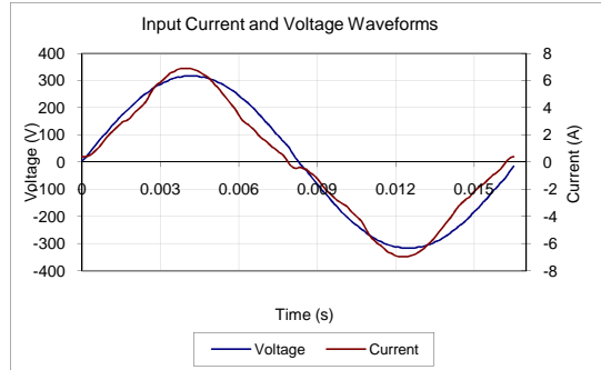
Input AC Current Waveform (ITHD = 15.98%, 100% Load)
